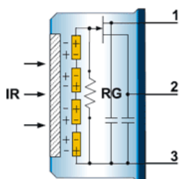
QUAD ELEMENT PYROELECTRIC INFRARED SENSOR
