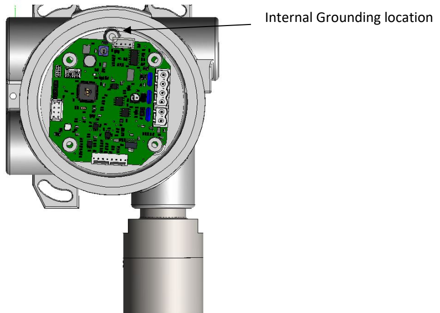
Diagram 8: Detector internal grounding screw location
