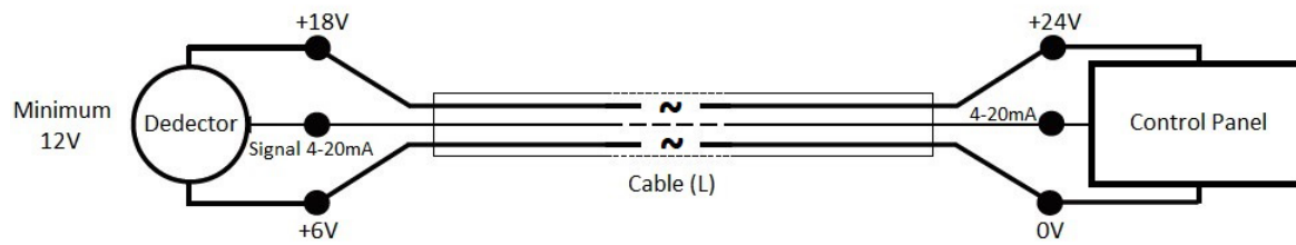
Diagram 6: Field cabling
