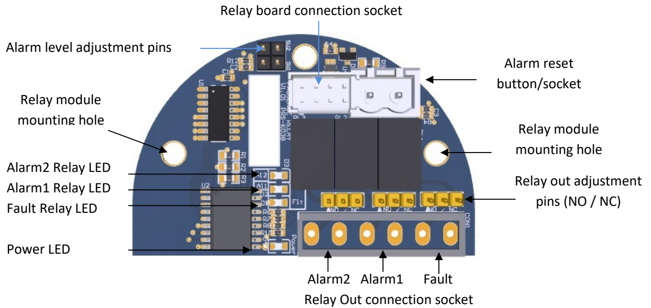
Diagram 11: Relay module
