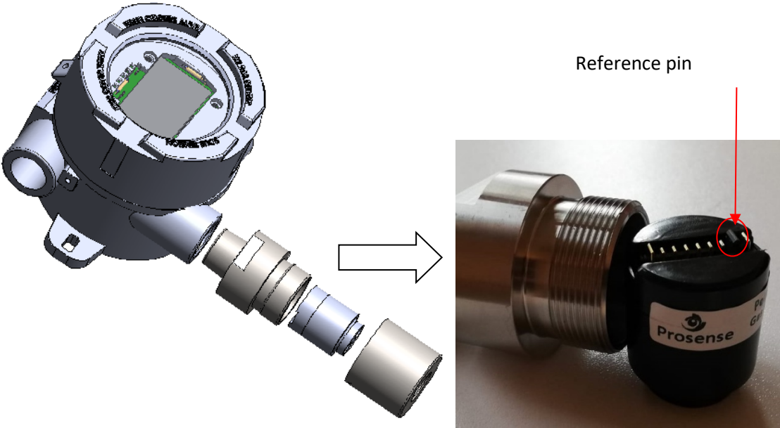
Diagram 14: PX Series sensor module
