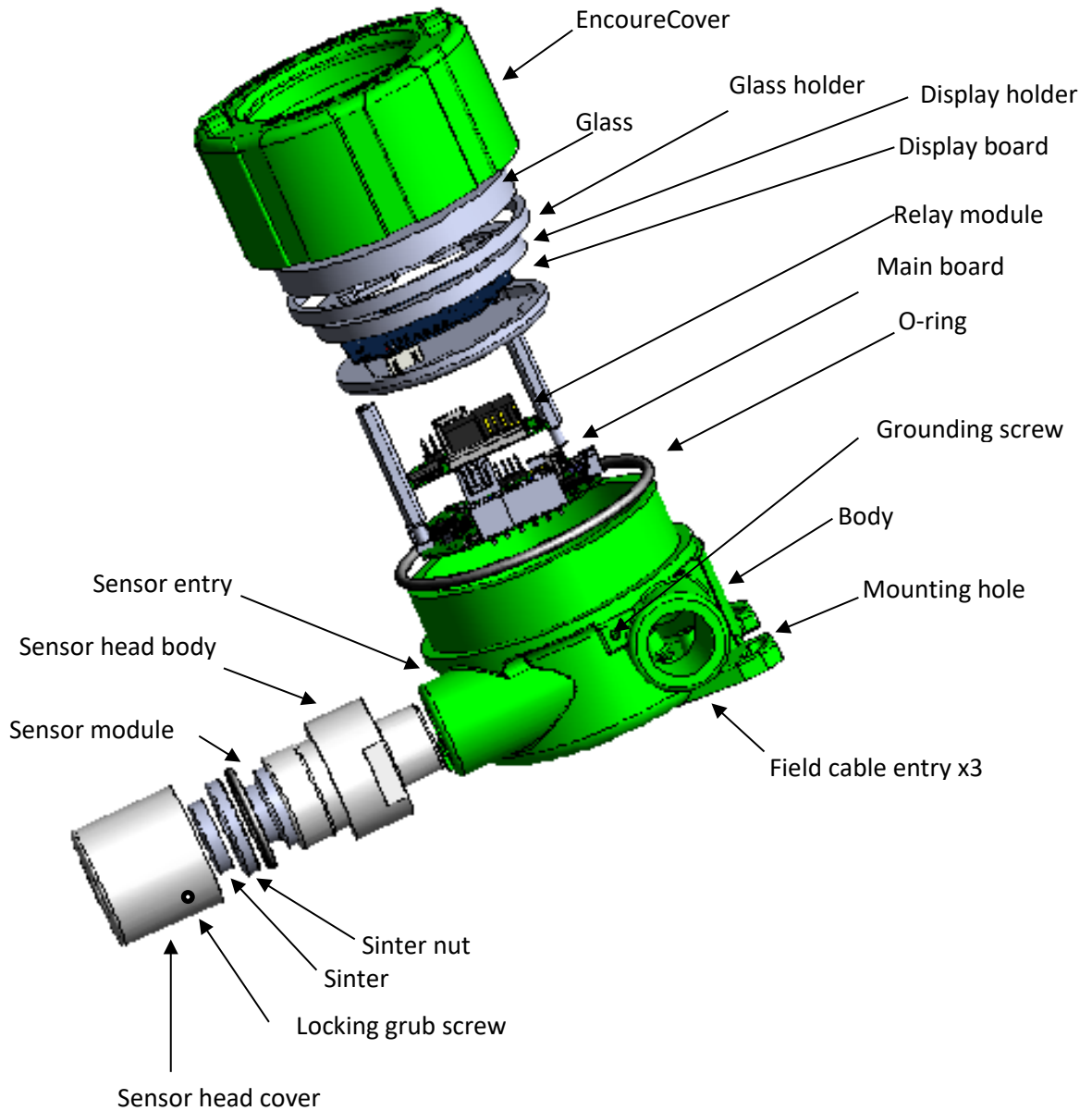
Diagram 1: Exploded view of PXD detector
