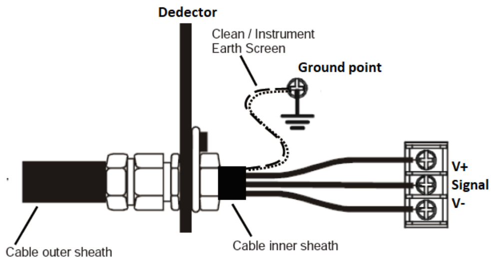
Diagram 7: Grounding
