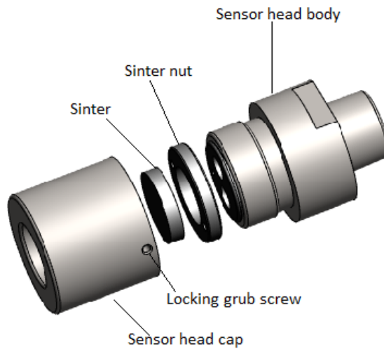
Diagram 4: Sensor Head components
