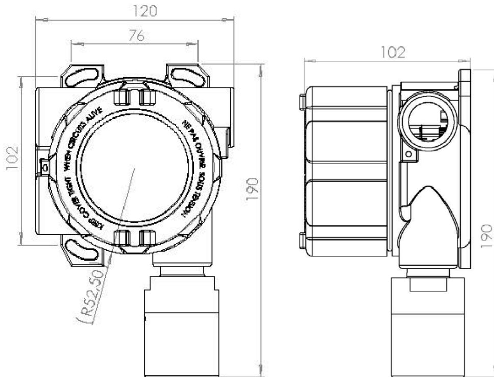
Diagram 2: Detector body and Sensor Head
