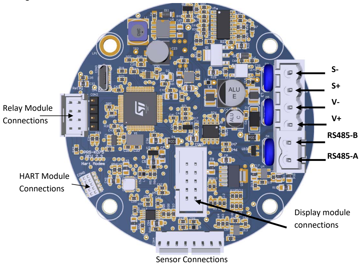
Diagram 10: Detector main board and connections
